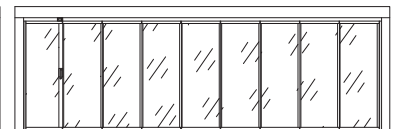
8 9 glass panel system Single module
